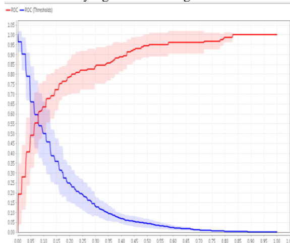
Gambar 7. AUC Model NB with GA
